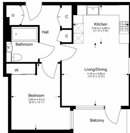
Ground Floor Total Gross Internal Area 49.5 Sq/m - 533 Sq/ft
