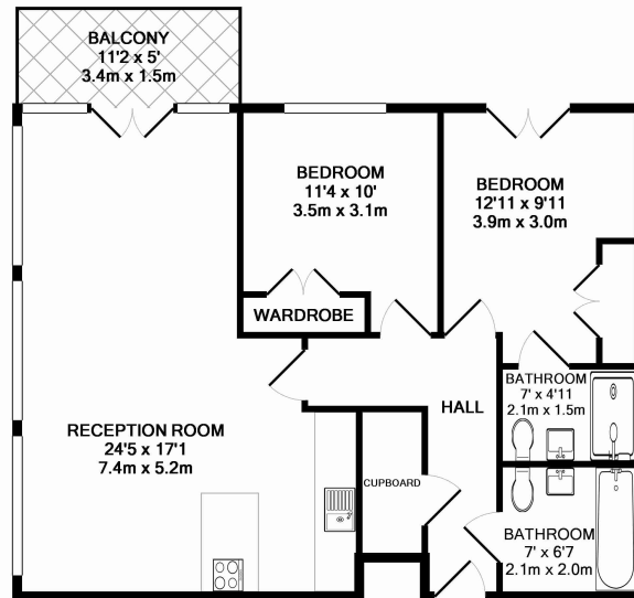
AVANT-GARDE APARTMENTS, AVANT GARDE PLACE, E1 TOTAL APPROX. FLOOR AREA 753 SQ.FT. (69.9 SQ.M.)
